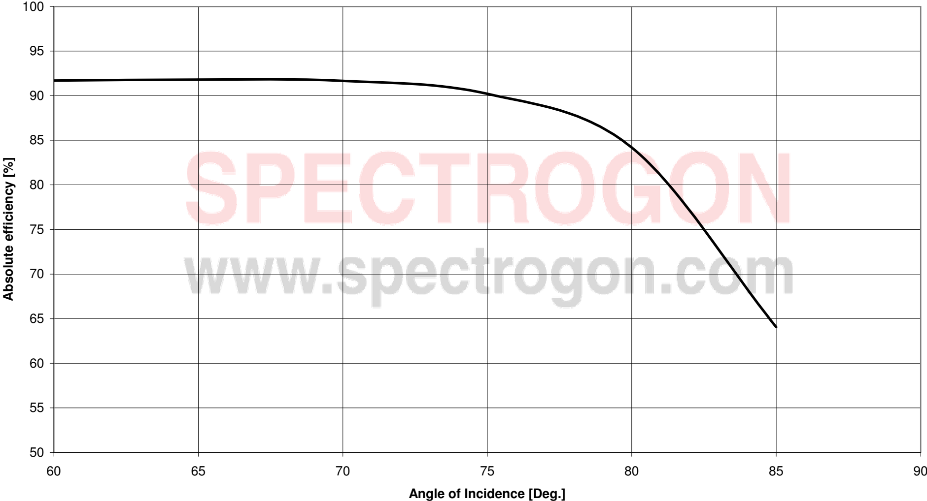
G 1200, Expected efficiency (TM/-1) @ 980 nm
