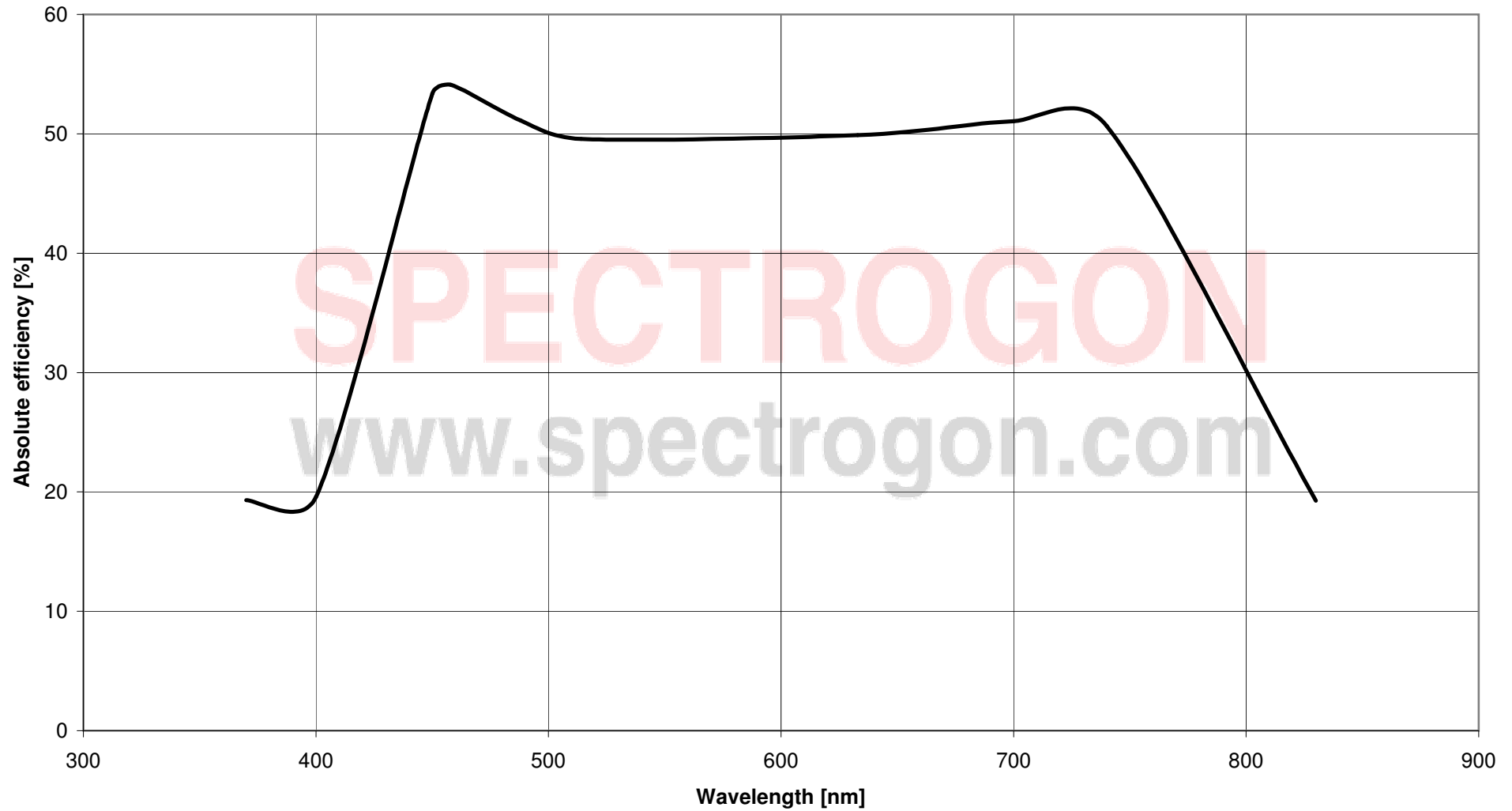
G 2400, Expected efficiency (TM/-1) @ AOI 85 Deg.
