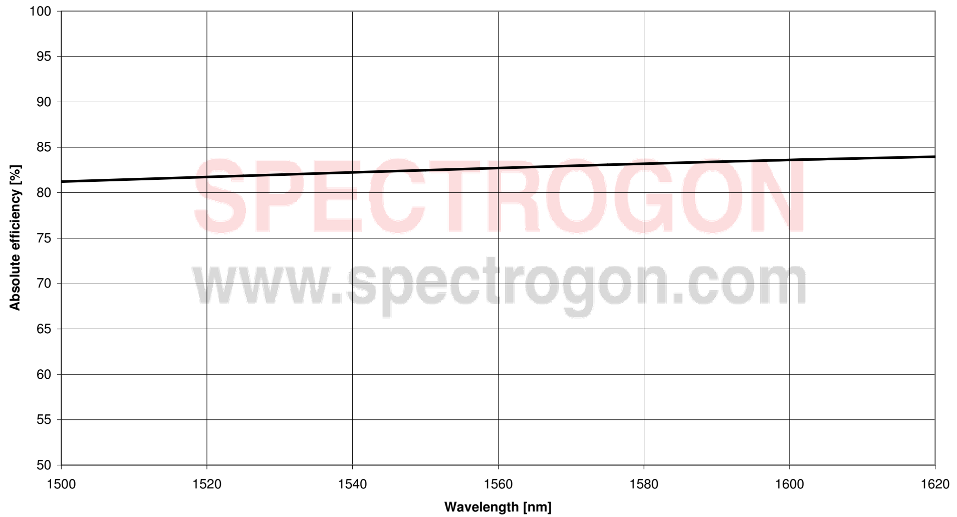
G 1100, Expected efficiency (TM/-1) @ AOI 80 deg
