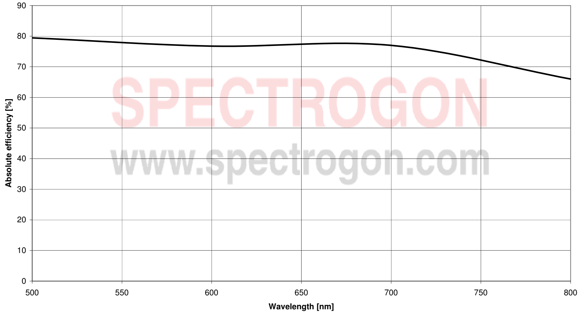
G 2400, Expected efficiency (TM/-1) @ AOI 75 deg
