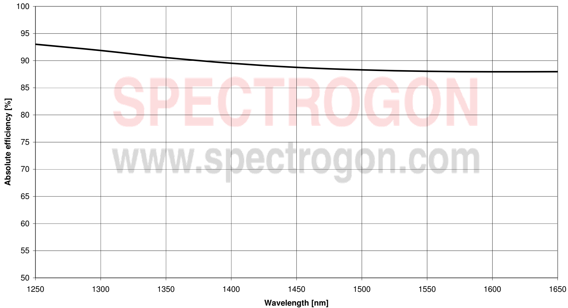
G 0900, Expected efficiency (TM-1) @ AOI 75 deg
