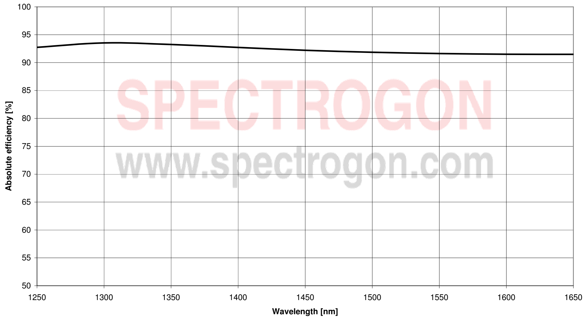
G 0900, Expected efficiency (TM/-1) @ AOI 70 deg.
