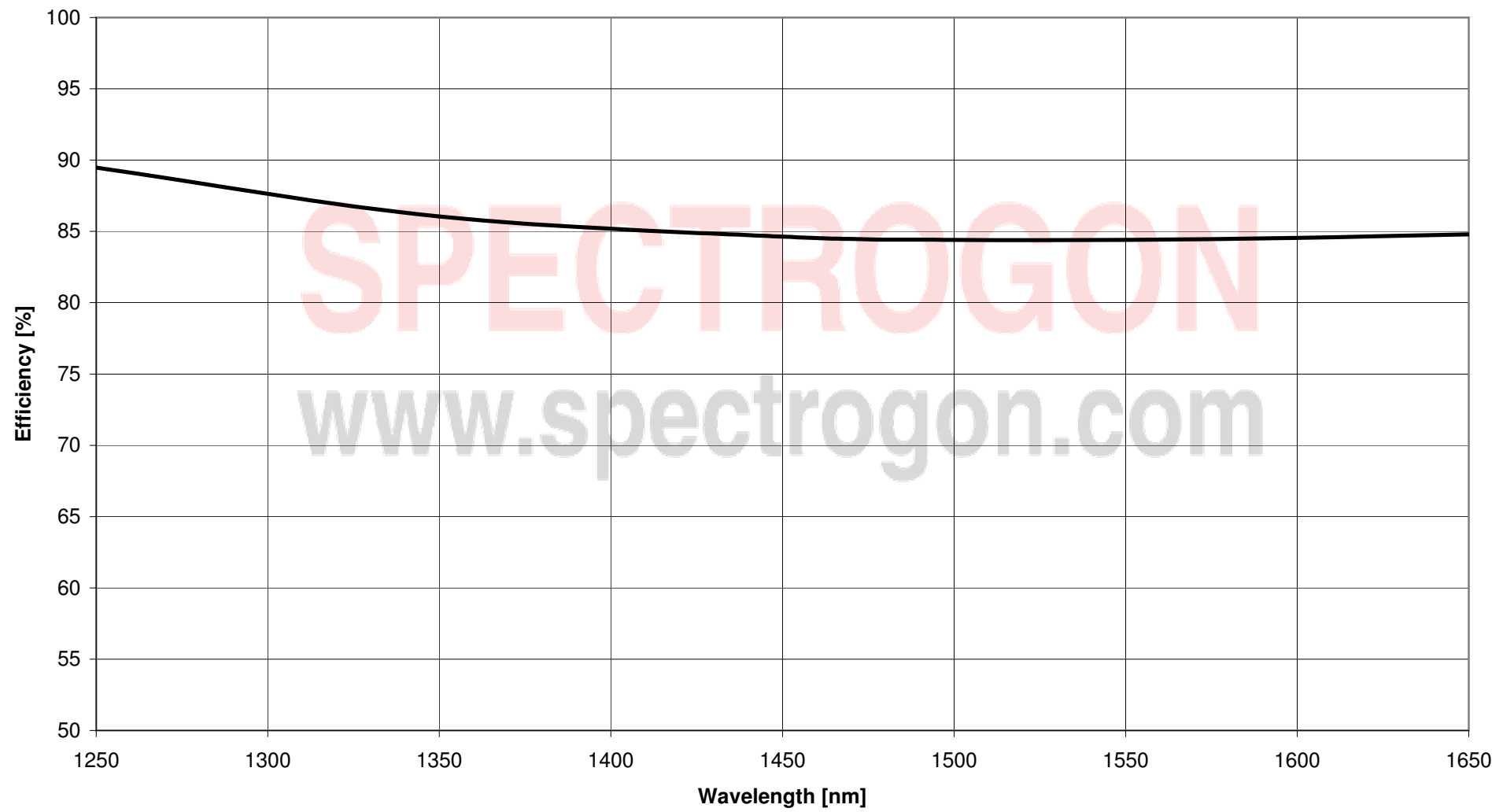
G 0900, Expected efficiency (TM/-1) @ AOI 78 deg
